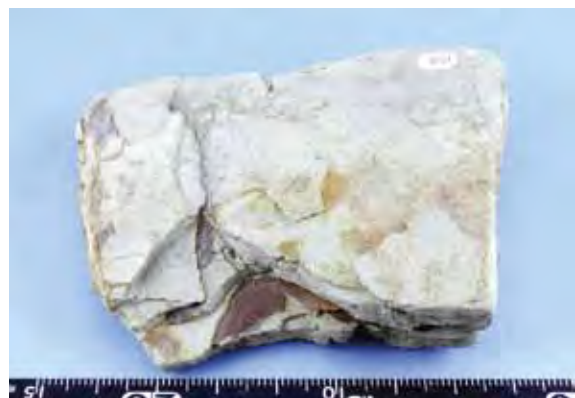
GR-128 頁岩 Shale
