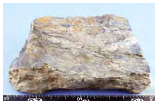
GR-235 絹雲母千枚岩 Sericite Phyllite
